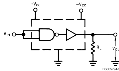
FIGURE 1. V_{IH} , V_{OL}
